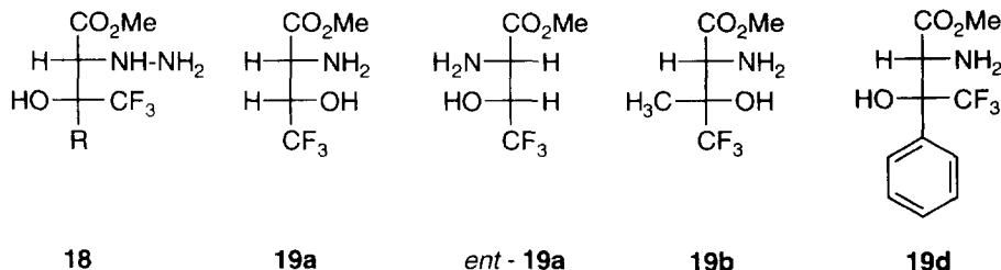
Chart 5. Fischer projections of some of the prepared \alpha -hydrazino- and \alpha -amino- \beta -hydroxycarboxylic acid derivatives containing CF 3 groups.
